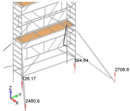
Reaction forces [N] - Plywood - Model L-000
