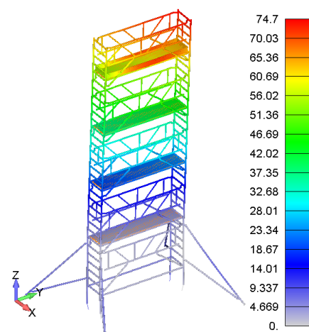
Displacements [mm] - Plywood - Model L-000
