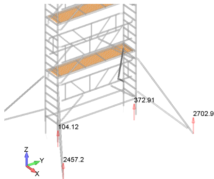
Reaction forces [N] - Fiberdeck - Model K-000
