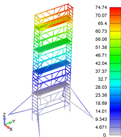
Displacements [mm] - Fiberdeck - Model K-000
