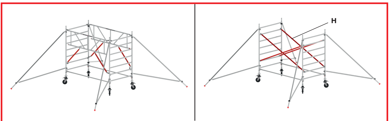
RS TOWER 52
