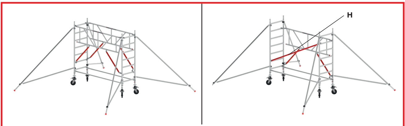
RS TOWER 52
