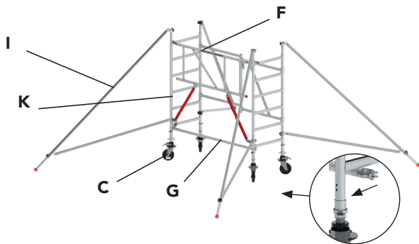
RS TOWER 54
